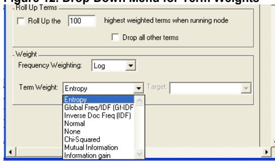
Figure 12. Drop-Down Menu for Term Weights
